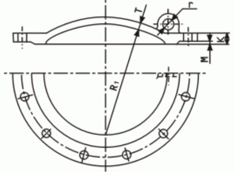
DN 150~1500mm (Apply to 7.5kg/cm 2 、10kg/cm 2 )
